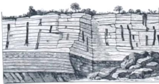
Fig. 442. — Vertical trees in the Coal Measures sandstone, St.-Étienne, France. From Cressler's Elements der Geologie .
